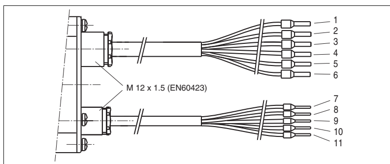
Terminal assignment BDM 7• with holding brake
