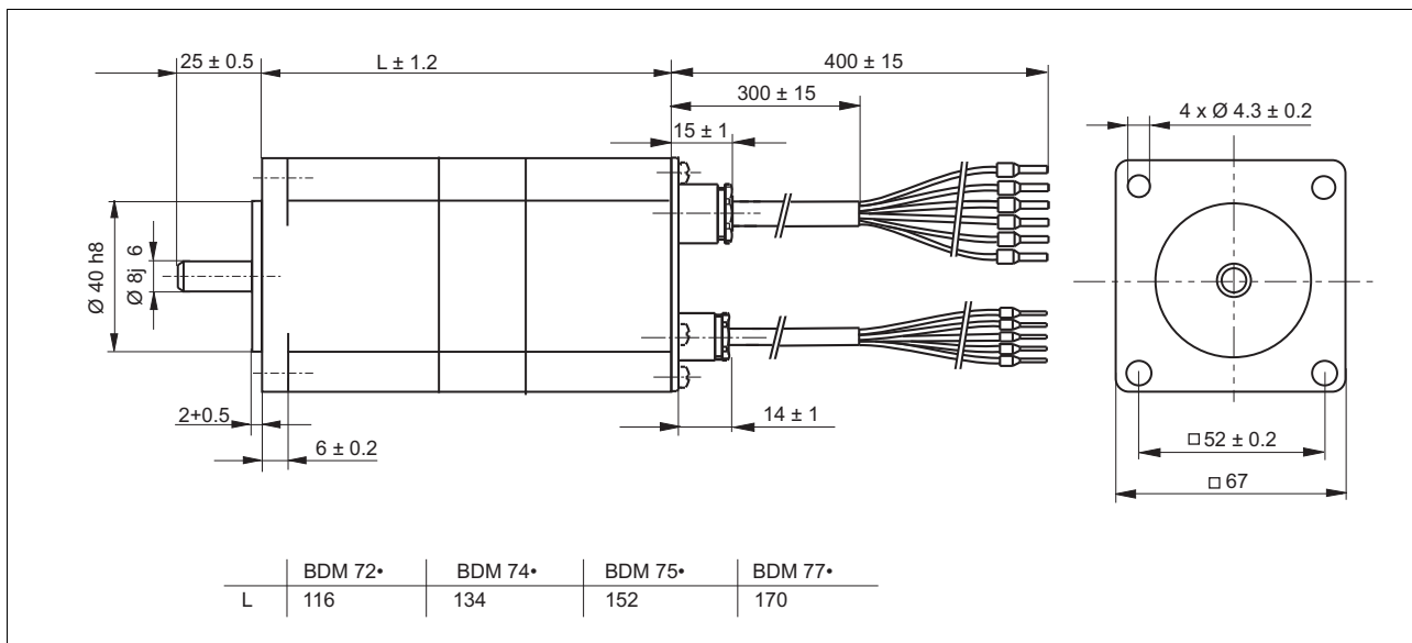
Dimensional drawing BDM 7• with holding brake
