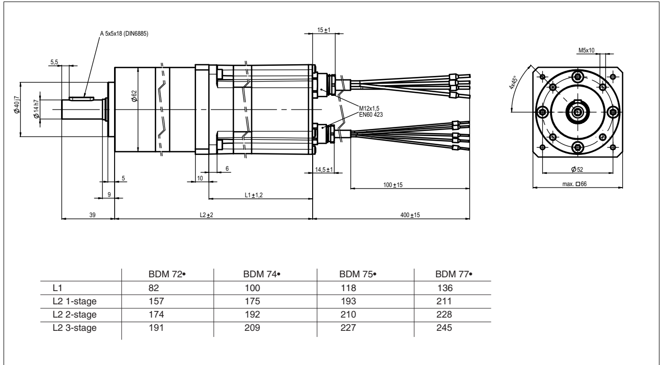
Dimensional drawing BDM 7• with yellow planetary gear PM62
