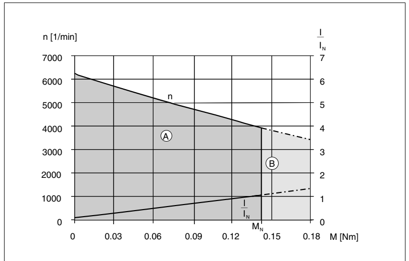
Torque characteristic BDM 433
