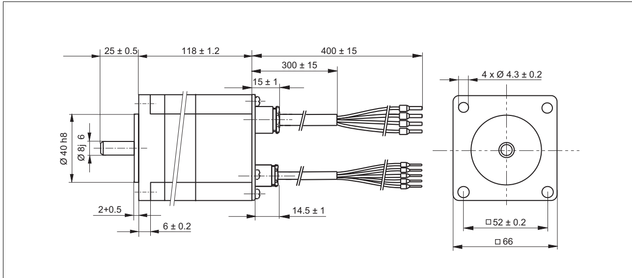
Dimensional drawing BDM 752
