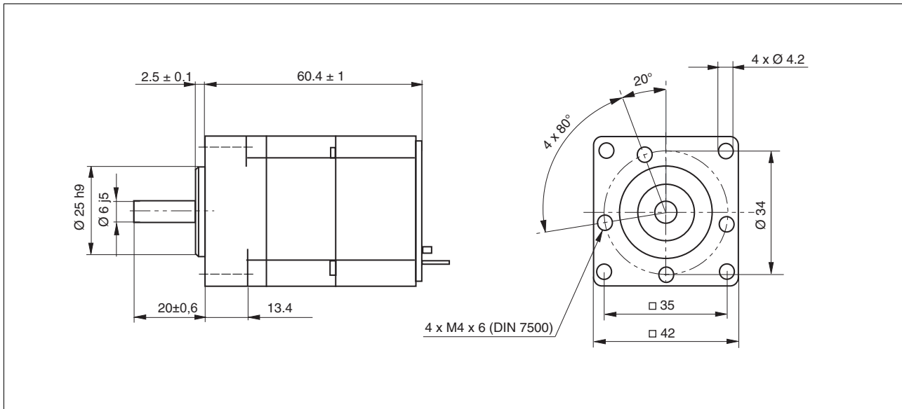
Dimensional drawing BDM 434
