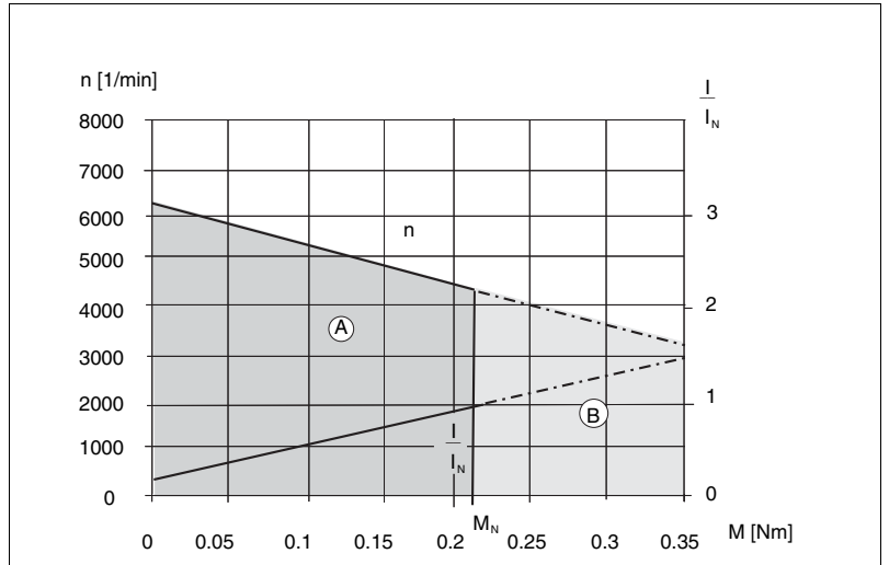
Torque characteristic BDM 454
